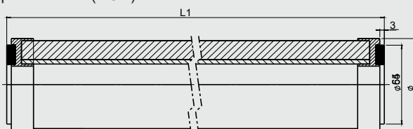
Type 10: Open flat seal (DOE)
