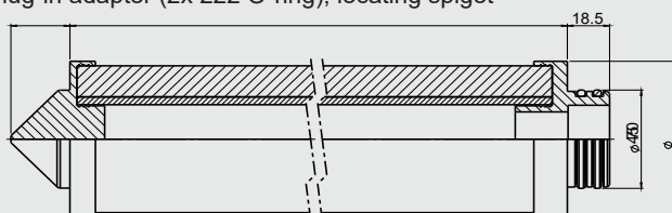
Type 7: Bayonet (2x 226 O-ring), locating spigot 25.5 L1
