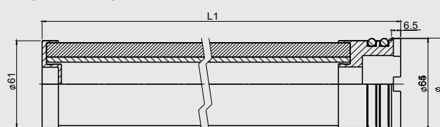
Type 12: Adapter for suspended elements
